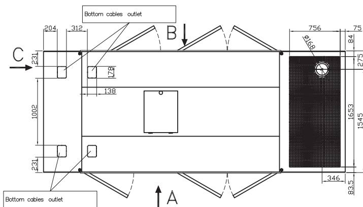
PIANTA/LAYOUT/ PLAN/PLAN
