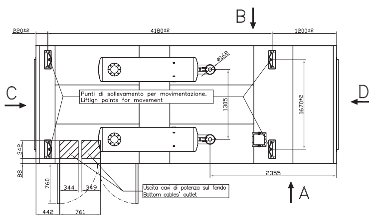
PIANTA/LAYOUT/ PLAN/PLAN
